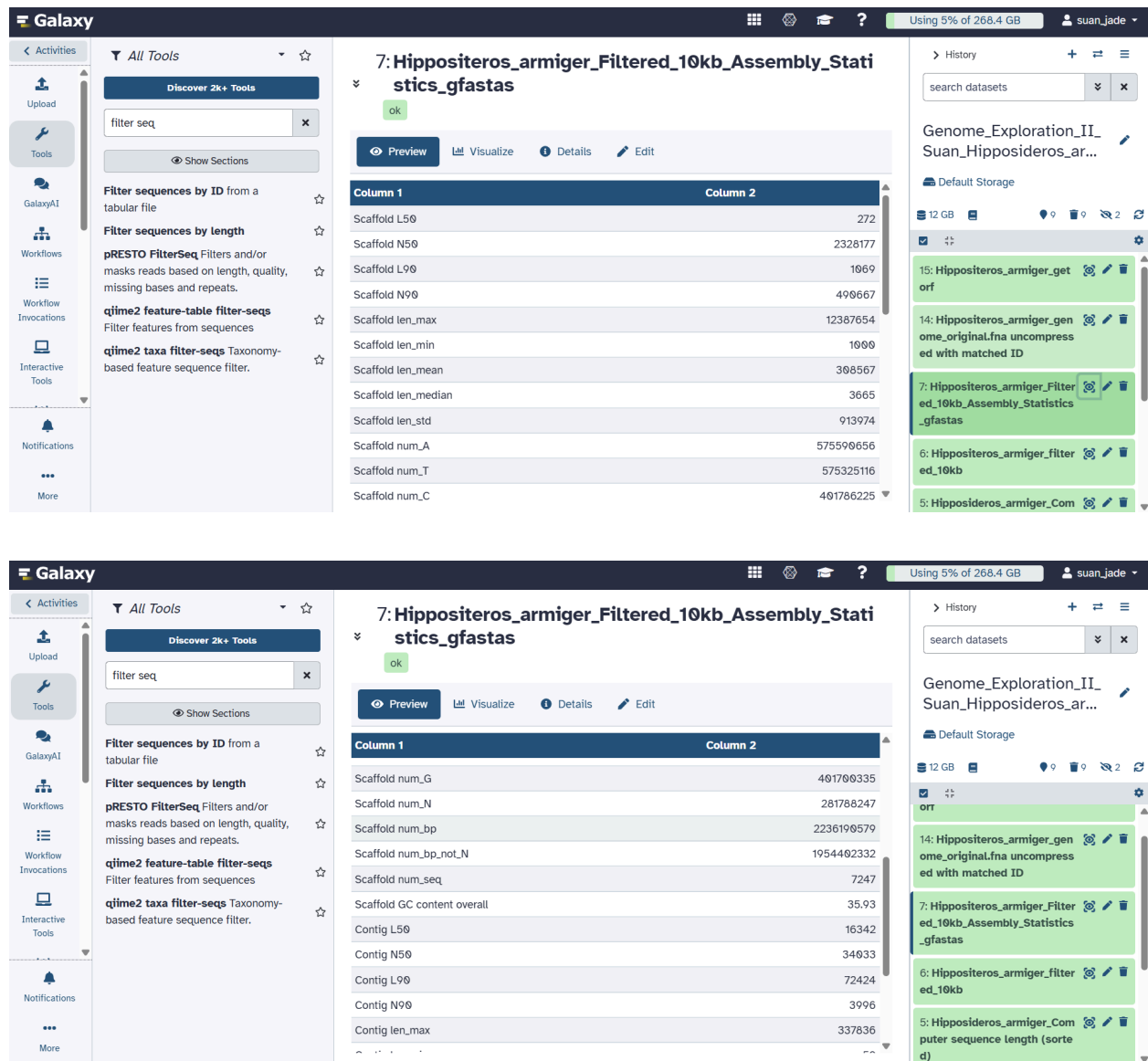
Figure 4b. Assembly statistics output from gfastats after filtering sequences \geq 10,000 bp. Comparison with the original genome shows that removing short sequences had almost no effect on total length, N50, and GC content, indicating short scaffolds contribute minimally to the overall assembly.
